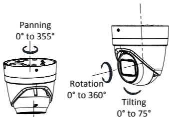
Figure 2-11 Adjust the View Angle
