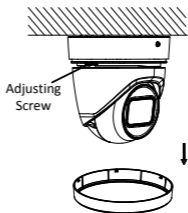
Figure 2-10 Loosen the Adjusting Screw
