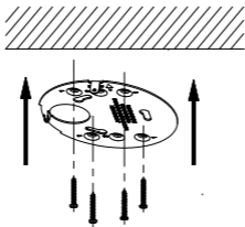
Figure 2-6 Secure the Adapter to the Ceiling
