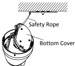
Figure 2-7 Hook the Camera to the Adapter
