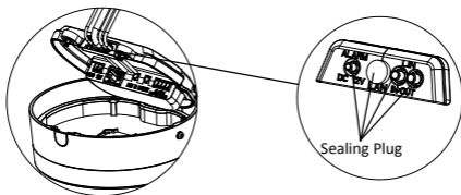
Figure 2-8 Route the Cables
