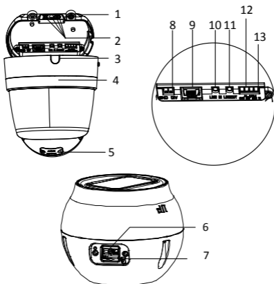
Figure 1-1 Overview of the Camera
