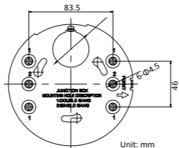
Figure 2-5 Drill Holes in the Ceiling
