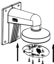
Figure 2-14 Secure the Adapter
